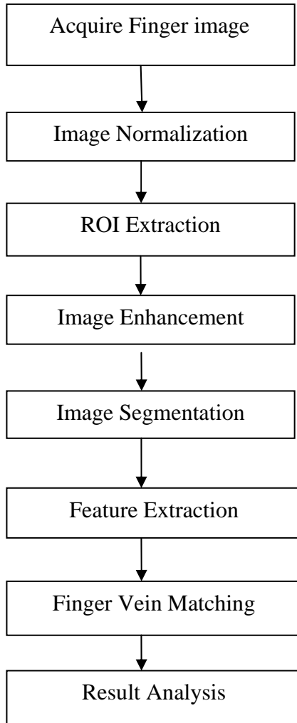
Figure 2: Flow Chart of Proposed Work.
